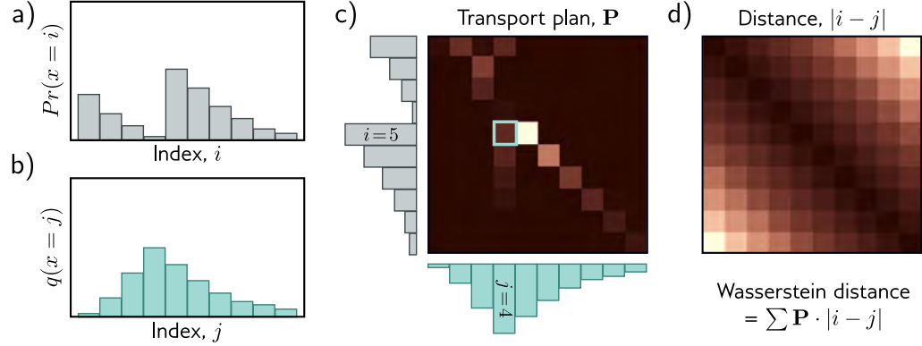
Figure 15.8 Wasserstein or earth mover's distance. a) Consider the discrete distribution Pr(x=i) . b) We wish to move the probability mass to create the target distribution q(x=j) . c) The transport plan \mathbf{P} identifies how much mass will be moved from i to j . For example, the cyan highlighted square p_{54} indicates how much mass will be moved from i=5 to j=4 . The elements of the transport plan must be non-negative, the sum over j must be Pr(x=i) , and the sum over i must be q(x=j) . Hence \mathbf{P} is a joint probability distribution. d) The distance matrix between elements i and j . The optimal transport plan \mathbf{P} minimizes the sum of the pointwise product of \mathbf{P} and the distance matrix (termed the Wasserstein distance). Hence, the elements of \mathbf{P} tend to lie close to the diagonal where the distance cost is lowest. Adapted from Hermann (2017).
