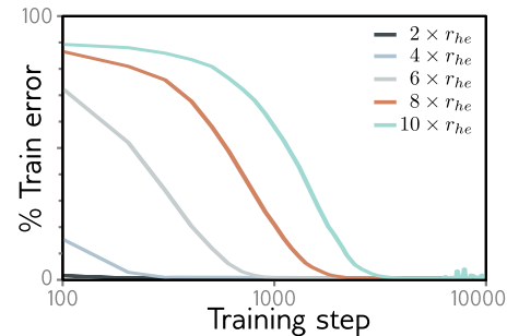
Figure 20.4 Initialization and fitting. A three-layer fully connected network with 200 hidden units per layer was trained on 1000 MNIST examples with AdamW using one-hot targets and mean-squared error loss. It takes longer to fit networks when larger multiples of He initialization are used, but this doesn't change the outcome. This may simply reflect the extra distance that the weights must move. Adapted from Liu et al. (2023c).
