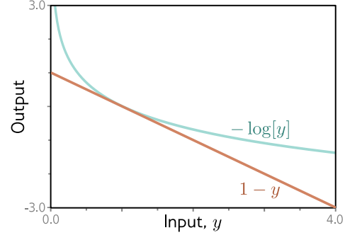
Figure C.6 Lower bound on negative logarithm. The function 1 - y is always less than the function -\log[y] . This relation is used to show that the Kullback-Leibler divergence is always greater than or equal to zero.
