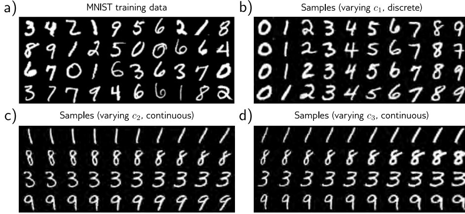
Figure 15.15 InfoGAN for MNIST. a) Training examples from the MNIST database, which consists of 28 \times 28 pixel images of handwritten digits. b) The first attribute c_1 is categorical with 10 categories; each column shows samples generated with one of these categories. The InfoGAN recovers the ten digits. The attribute vectors c_2 and c_3 are continuous. c) Moving from left to right, each column represents a different value of c_2 while keeping the other latent variables constant. This attribute seems to correspond to the orientation of the character. d) The third attribute seems to correspond to the thickness of the stroke. Adapted from Chen et al. (2016b).
