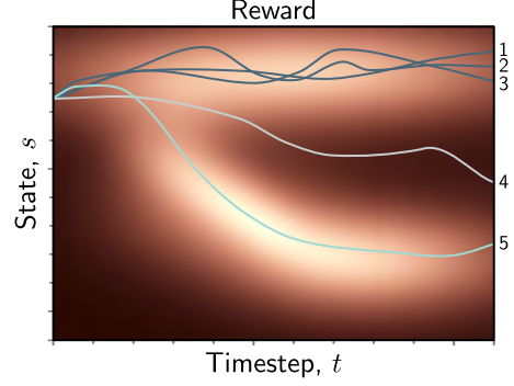
Figure 19.15 Policy gradients. Five episodes for the same policy (brighter indicates higher reward). Trajectories 1, 2, and 3 generate consistently high rewards, but similar trajectories already frequently occur with this policy, so there is no need to change. Conversely, trajectory 4 receives low rewards, so the policy should be modified to avoid producing similar trajectories. Trajectory 5 receives high rewards and is unusual. This will cause the largest change to the policy under equation 19.25.
