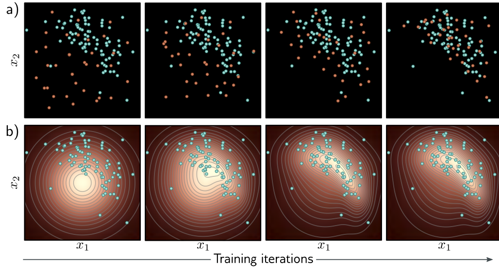
Figure 14.2 Fitting generative models a) Generative adversarial models provide a mechanism for generating samples (orange points). As training proceeds (left to right), the loss function encourages these samples to become progressively less distinguishable from real examples (cyan points). b) Probabilistic models (including variational autoencoders, normalizing flows, and diffusion models) learn a probability distribution over the training data. As training proceeds (left to right), the likelihood of the real examples increases under this distribution, which can be used to draw new samples and assess the probability of new data points.
